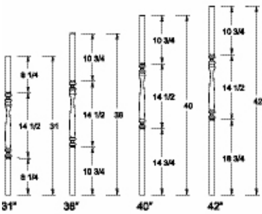
F-5801-H 1-1/4" Square
