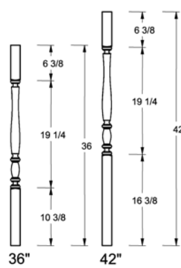
F-5905 1 3/4" Square
