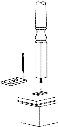
JP-3005 Keylock
