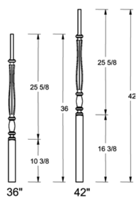
F-5911 FL 1 3/4" Tapered Top
