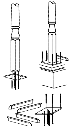
JP-306 Mounting Plate
