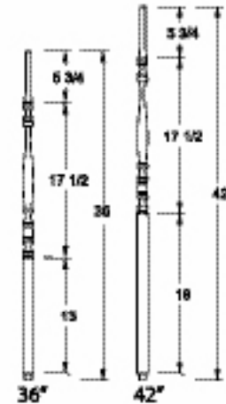
F-5610-H 1-1/4" Square
