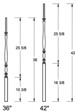
F-5019 1 1/4" Tapered Top
