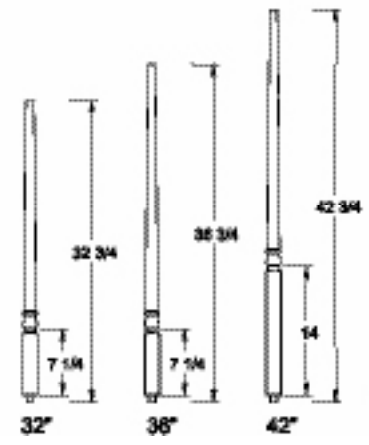
F-5315-H 1-5/8" Square
