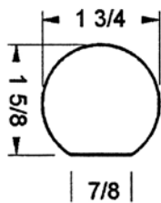
JP-6040
