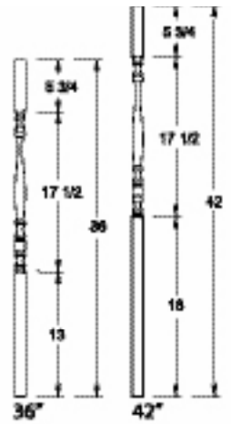
F-5105-H 1-1/4" Square
