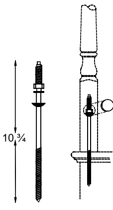
JP-3008 Sure-Tite
