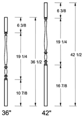
F-5109 1 1/4" Square
