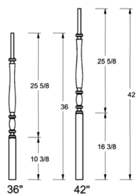
F-5911 1 3/4" Tapered Top
