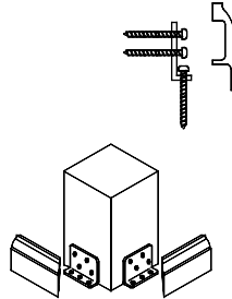
JP-319 L-Anchor
