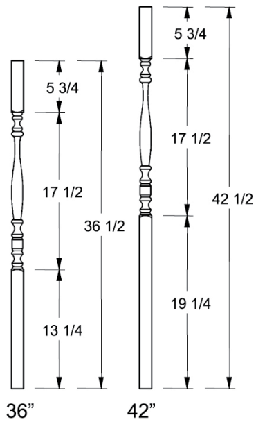
F-5105-O 1-1/4" Square
