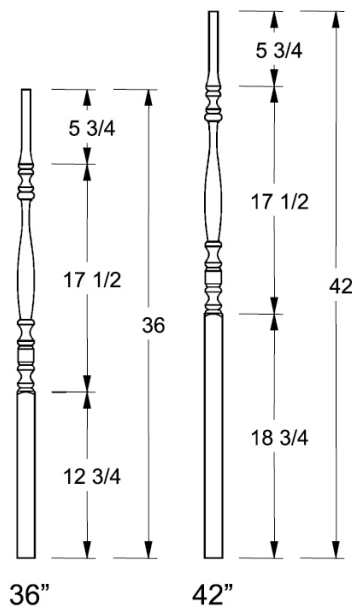
F-5610-O 1-1/4" Square
