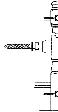
JP-378 Newel & Rail Fastener
