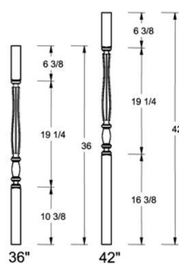
F-5905 FL 1 3/4" Square
